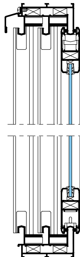
Sliding Windows Vertical section
