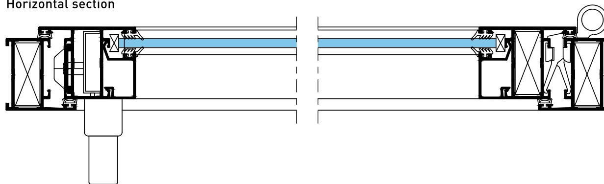
Casement Windows Horizontal section
