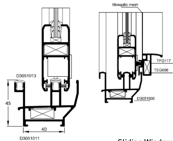
Sliding Windows Vertical section
