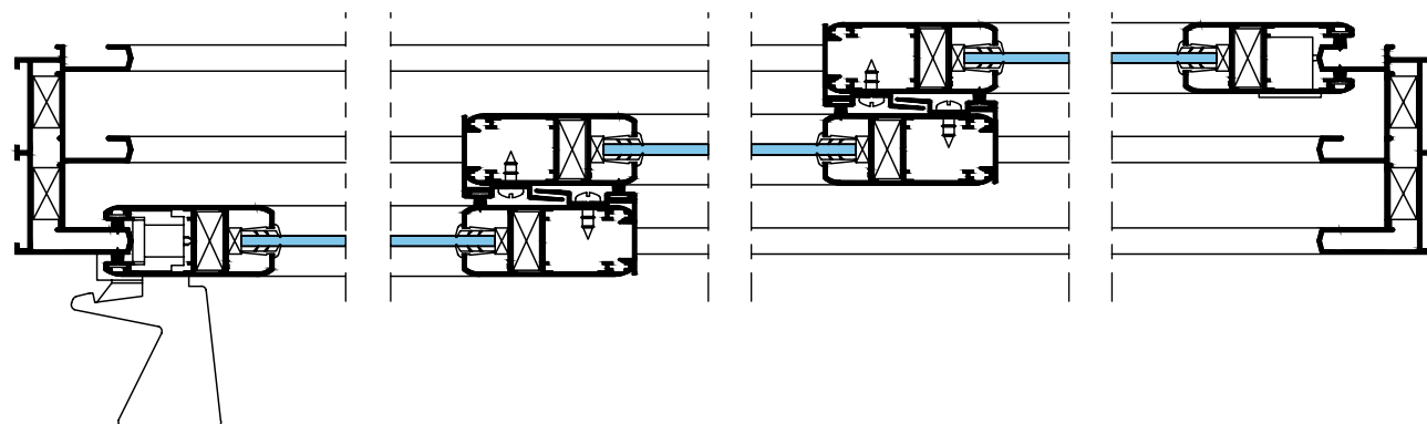
Sliding Windows Horizontal section
